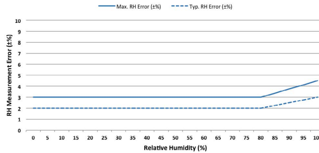
RH Accuracy
