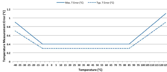
Temperature Accuracy
