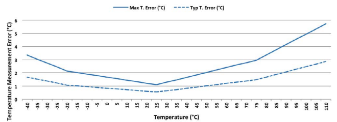
Temperature Accuracy
